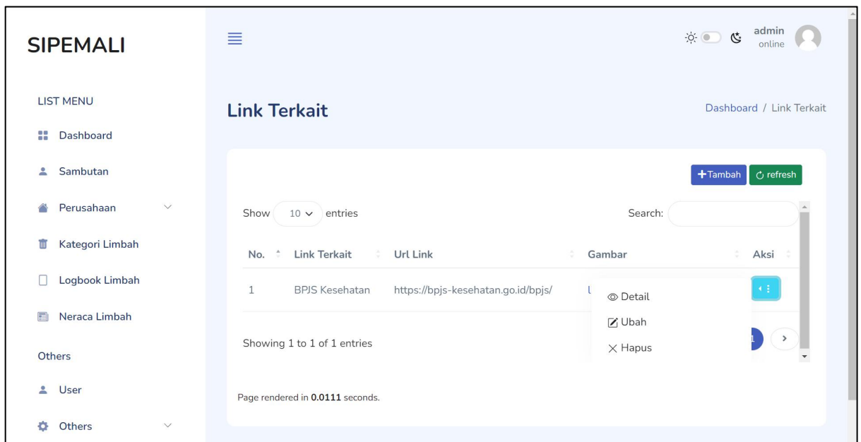
Gambar 50 Tombol Aksi
