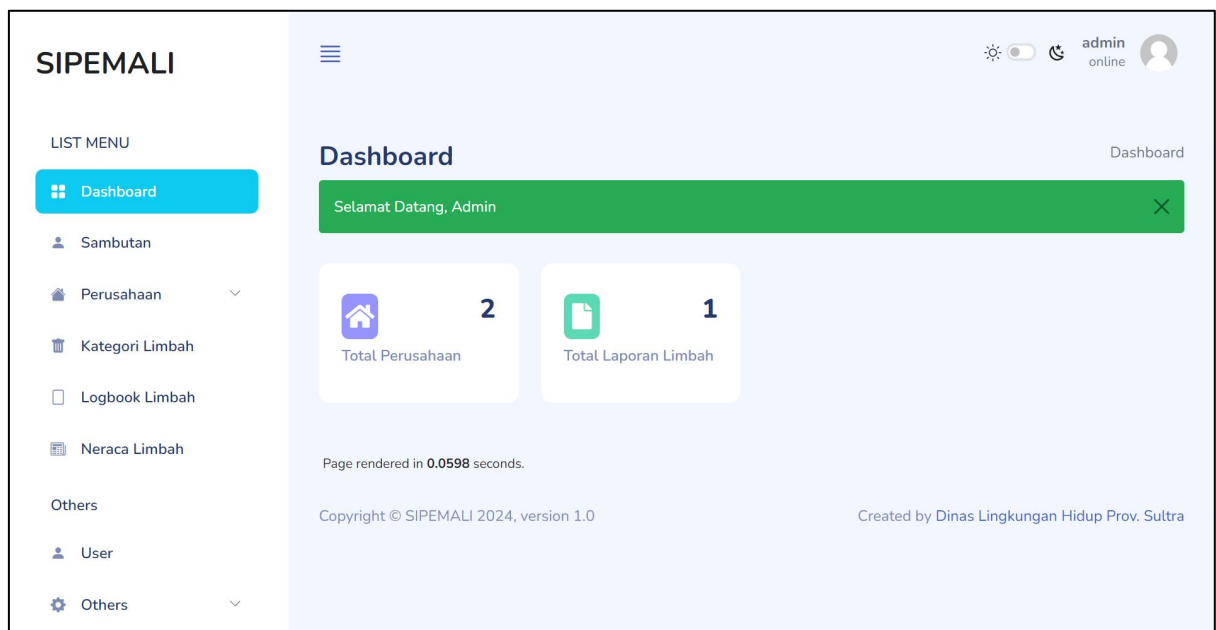
Gambar 12 Menu Dashboard
