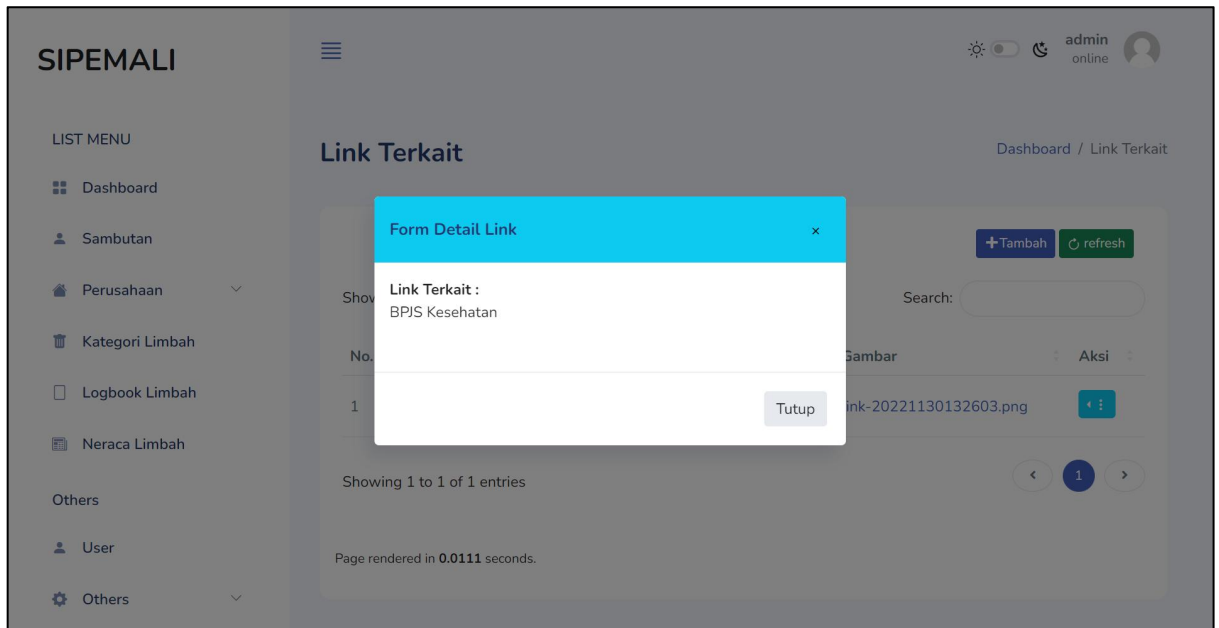
Gambar 51 Detail
