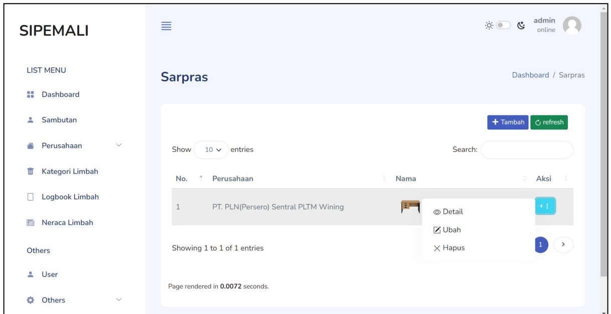
Gambar 28 Tombol Aksi
