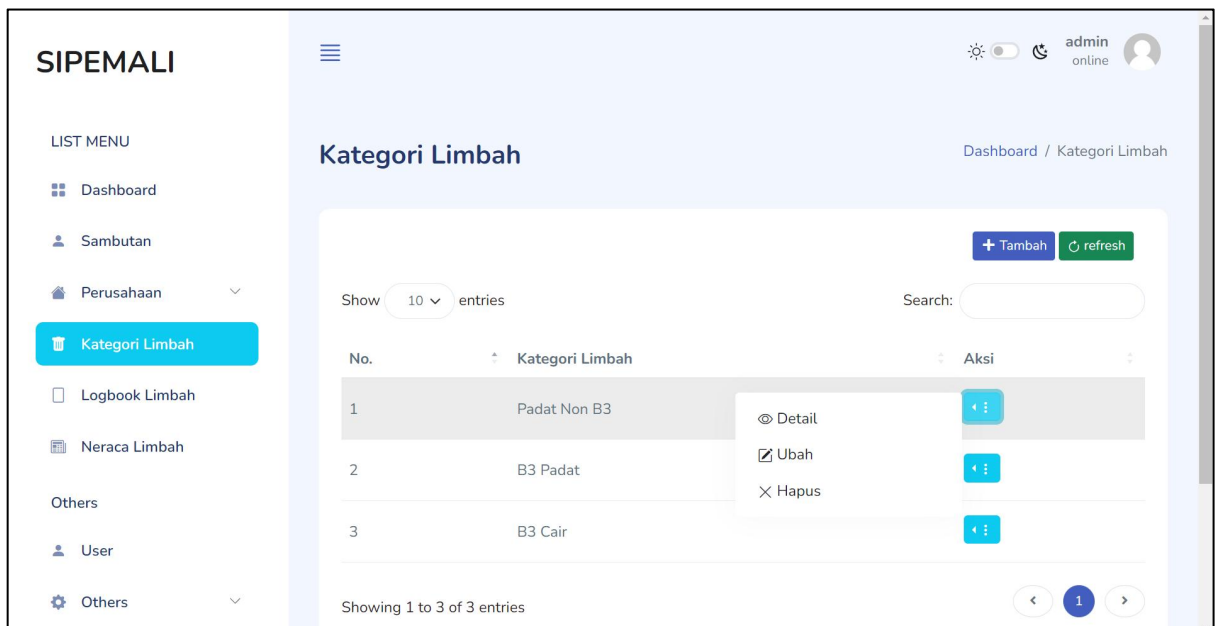
Gambar 34 Tombol Aksi
