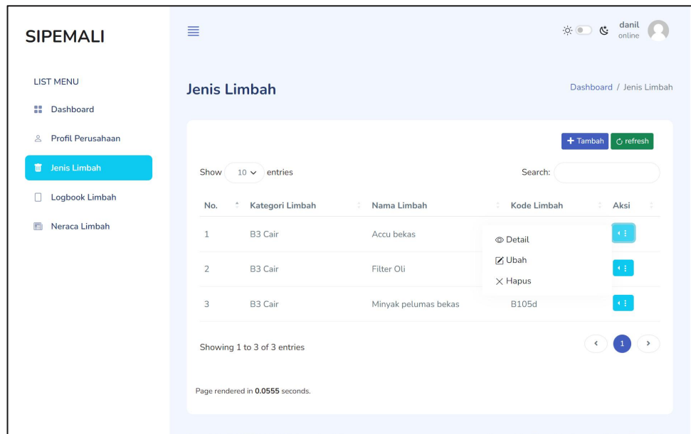
Gambar 64 Tombol Aksi
