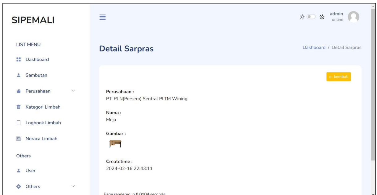
Gambar 29 Detail Sarpras
