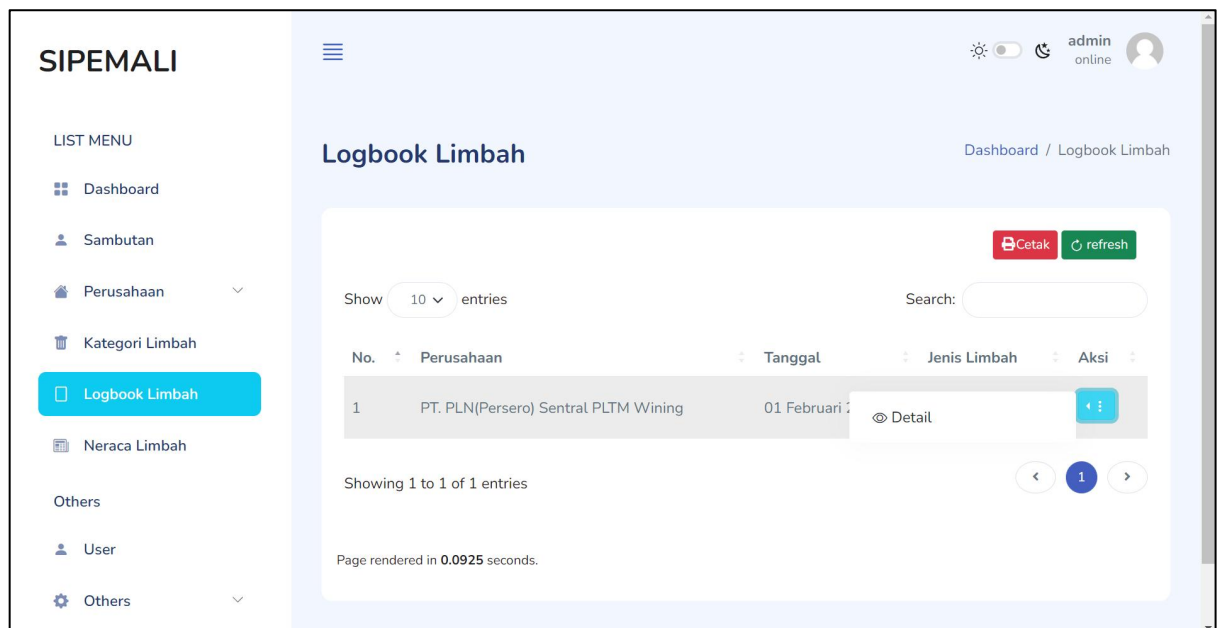
Gambar 40 Tombol Aksi
