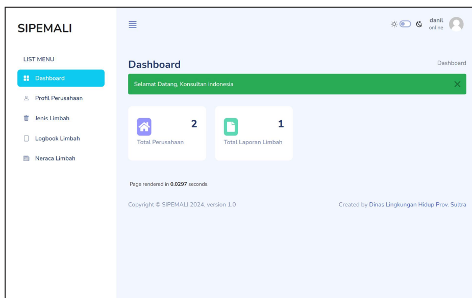
Gambar 60 Dashboard
