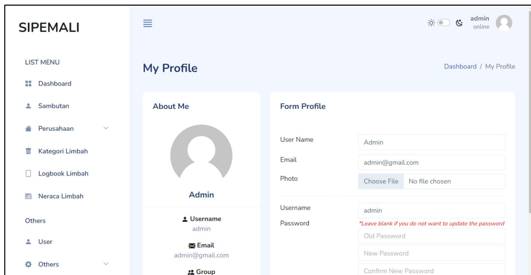
Gambar 59 Profile
