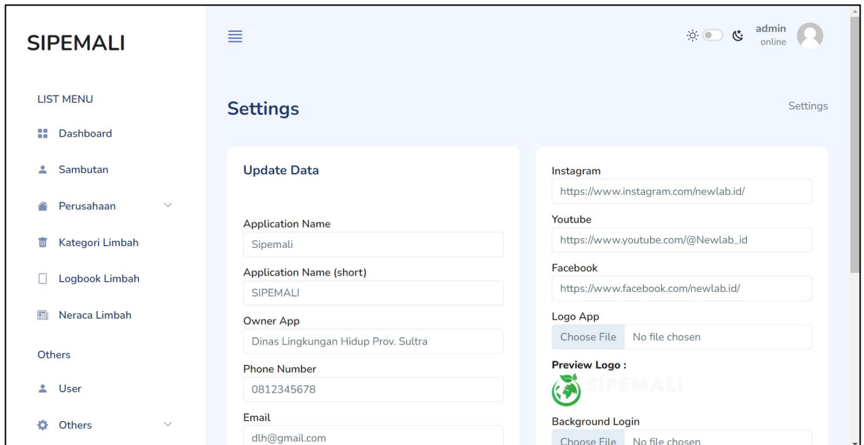
Gambar 47 Settings
