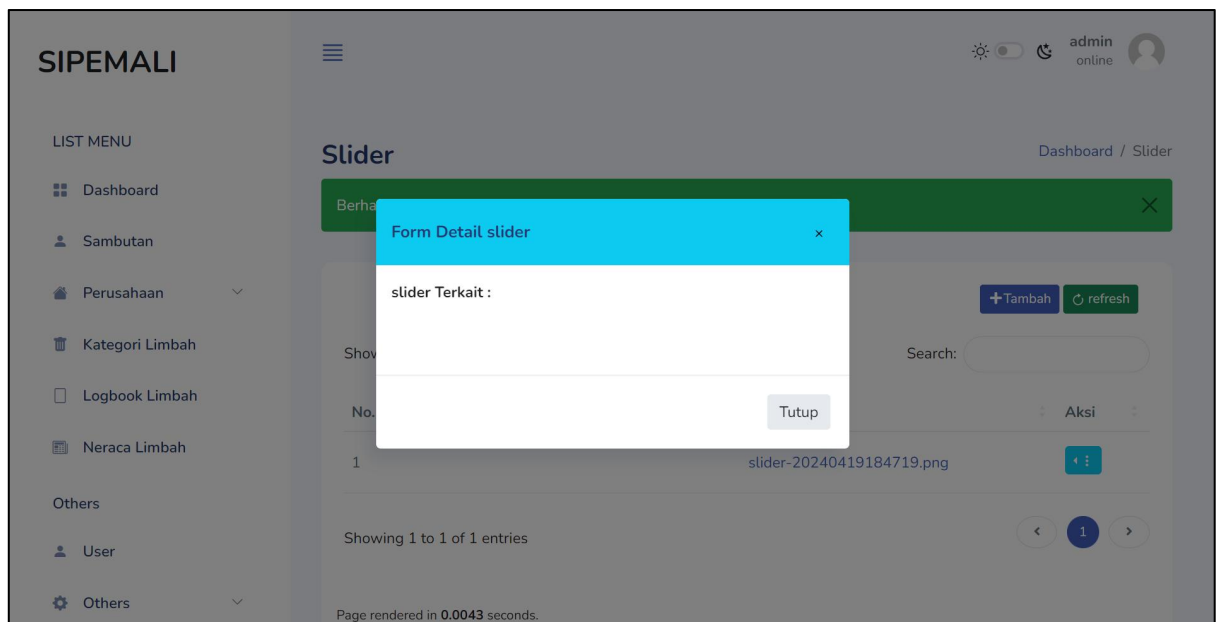
Gambar 56 Detail
