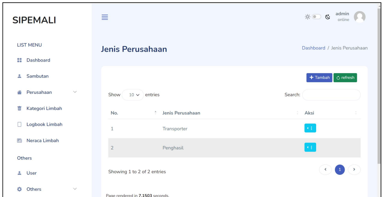
Gambar 16 Tombol Aksi
