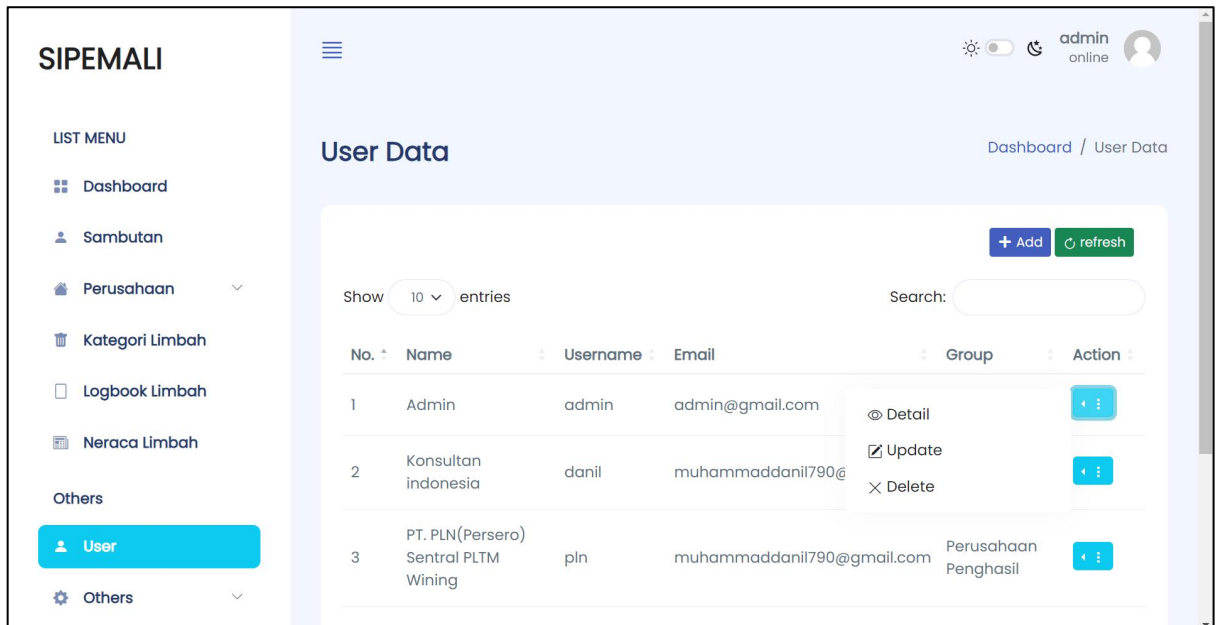
Gambar 46 Tombol Aksi
