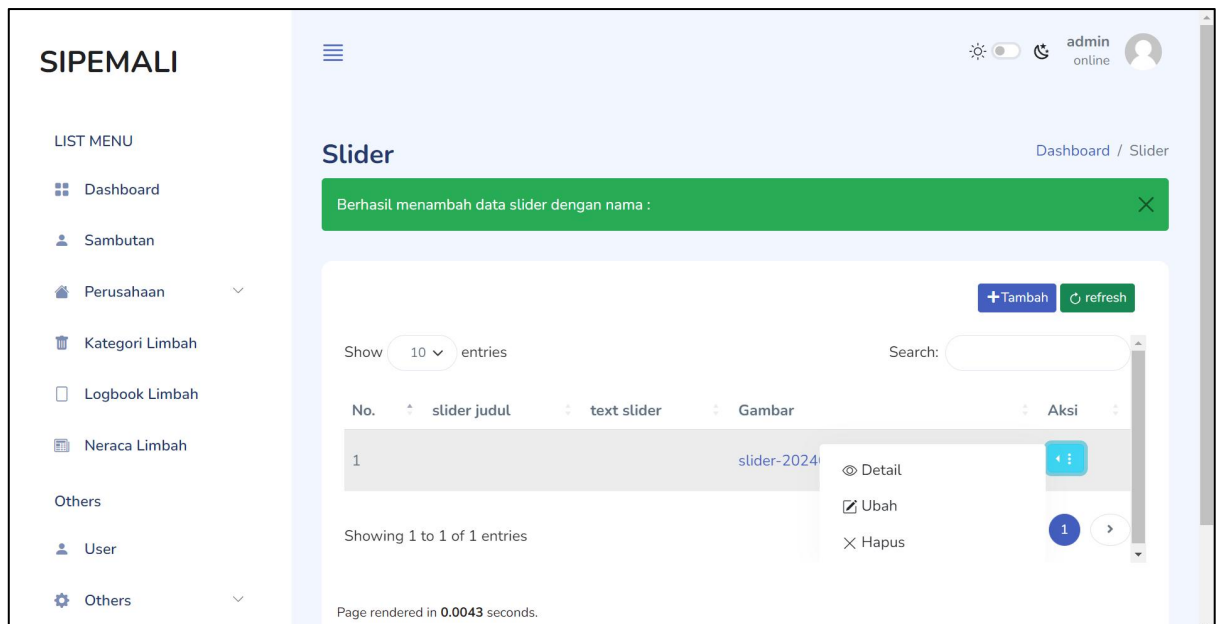
Gambar 55 Tombol Aksi
