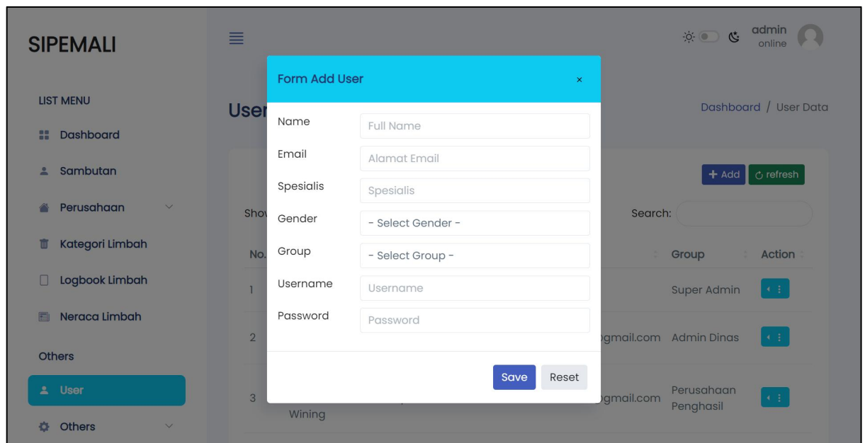
Gambar 45 tambah User
