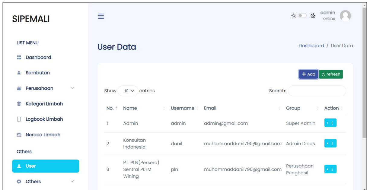
Gambar 44 Menu User
