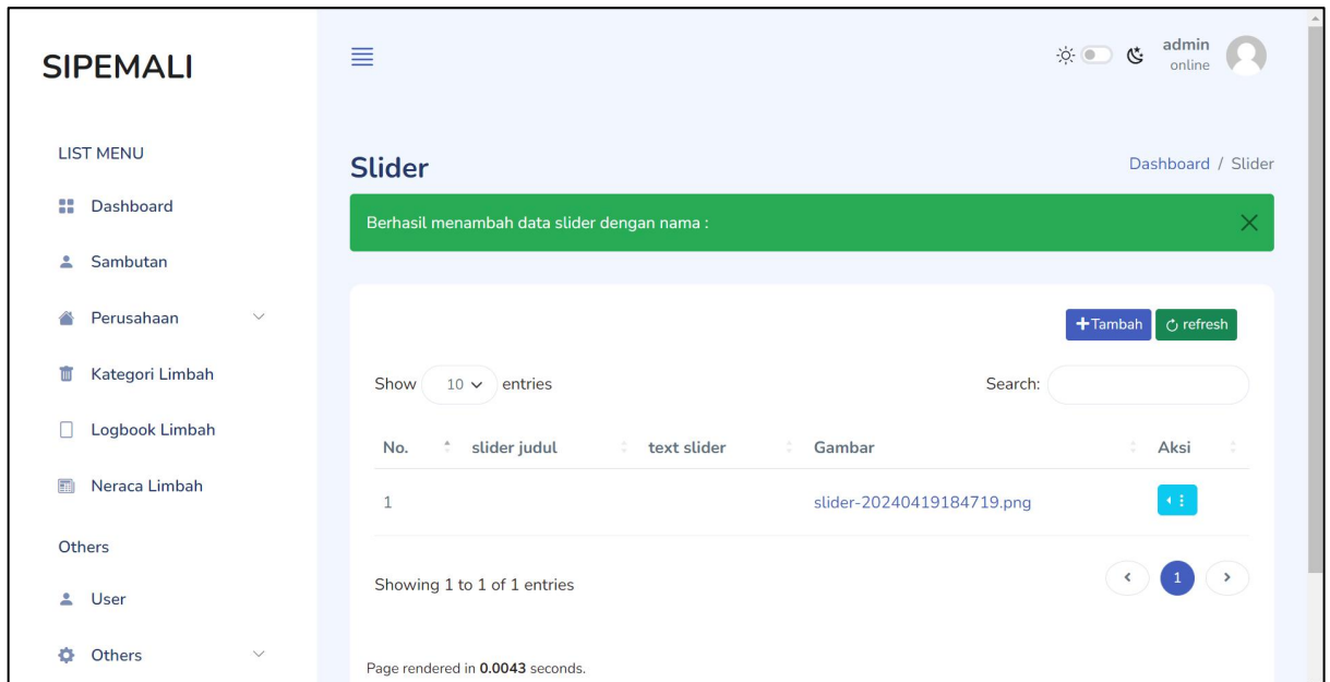
Gambar 53 Slider
